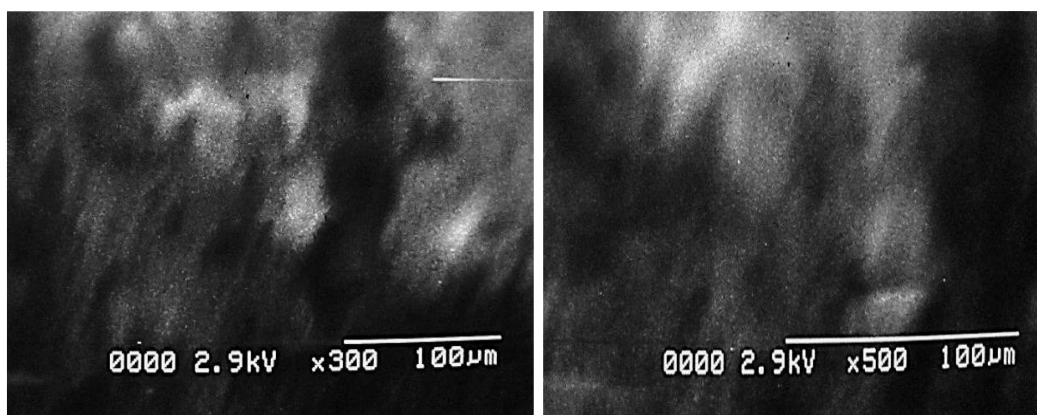
Figure 3. SEM images of starch/polyacrylamide composite containing 10% ZnSO 4 .
