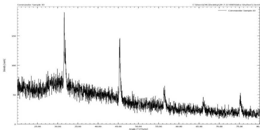
Figure 6. XRD of Starch-g-Polyacrylamide composite containing 1% ZnSO 4 salt. Five sharp peaks with high intensity show the strong interaction between composite and metal salt
