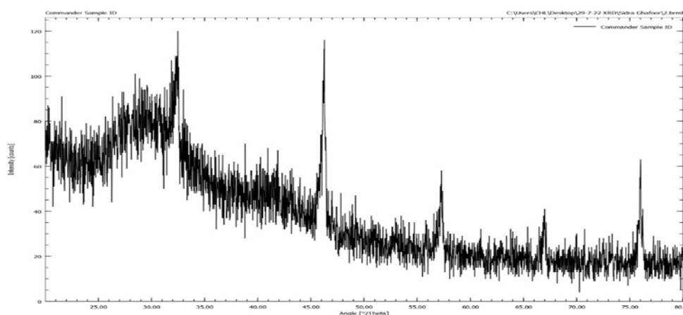
Figure 7. XRD of Starch-g-Polyacrylamide composite containing 10 % ZnSO 4 . Five sharp peaks than pure composite shows the interaction between composite and metal salt.
