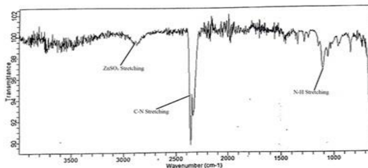
Figure 8. FTIR spectrum of composite containing 2.5 % ZnSO 4 .
