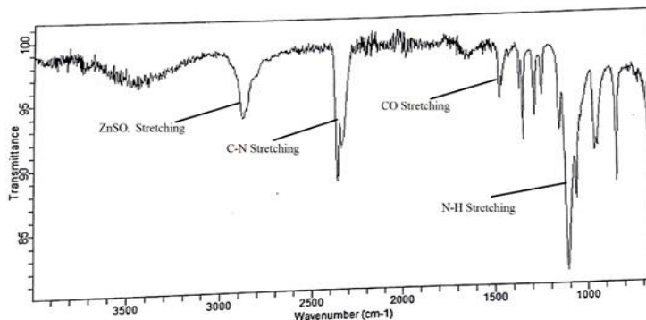
Figure 10. FTIR spectrum of composite containing 10 % ZnSO 4 .
