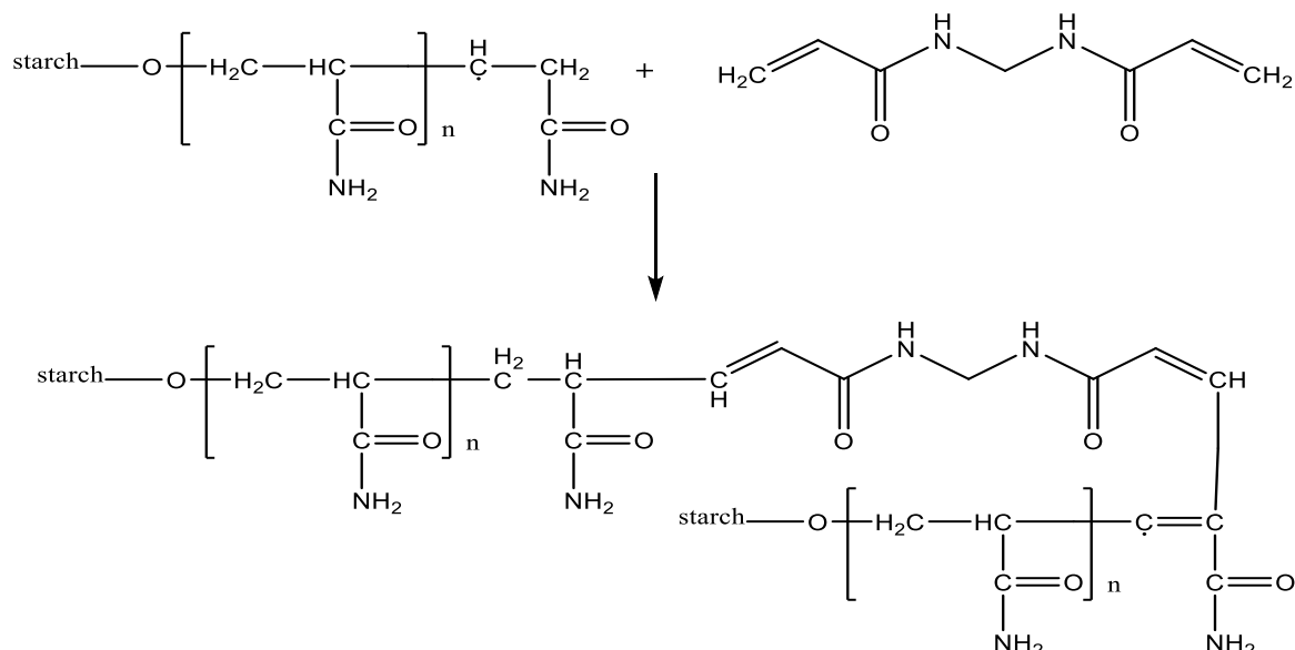
Figure 1. Mechanism for synthesis of starch-g-polyacrylamide composite.
