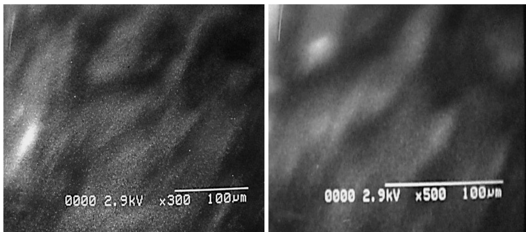
Figure 2. SEM images of starch/polyacrylamide (St-g-Pam) composite having uniform structure.
